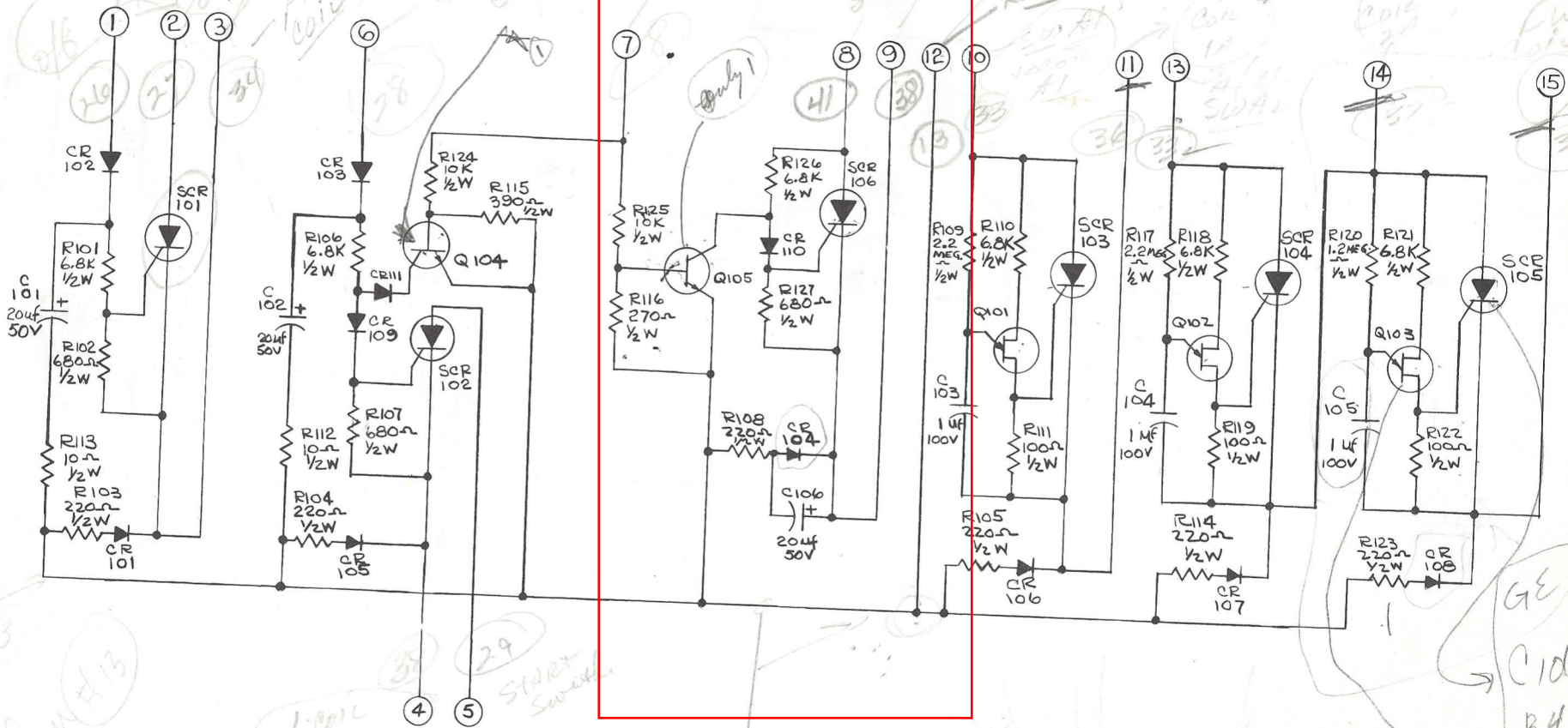
Fig. 5-8 26AE15 Card #1 (Control) Schematic
